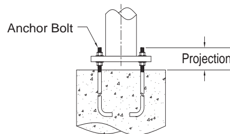
Base Detail
